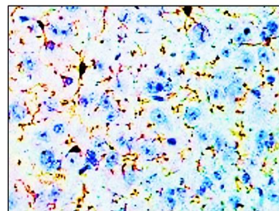
Mouse brain
